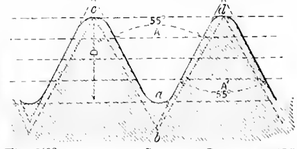
Fig. 5496. WHITWORTH STANDARD SCREW-THREADS. English and Continental standard.
